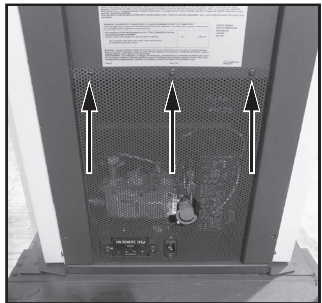
Figure 61: Rear screen removal.
