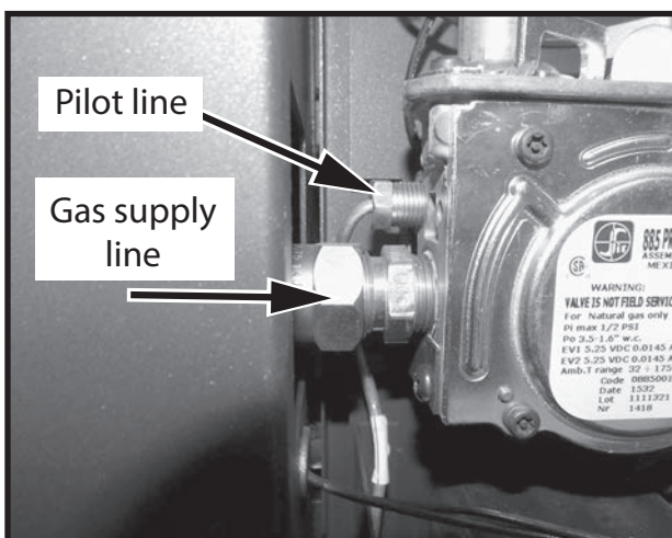
Figure 62: Gas line connections at gas valve.
