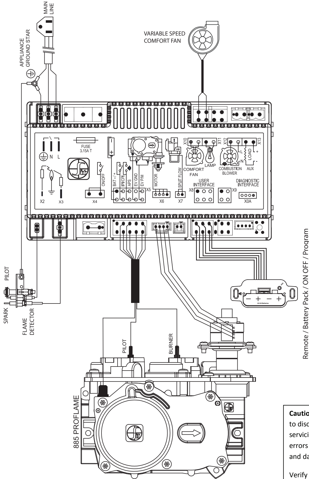
Figure 75: Electrical diagram for Mirage 18.
