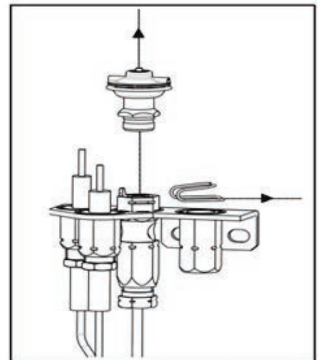
Figure 73: Pilot hood.
