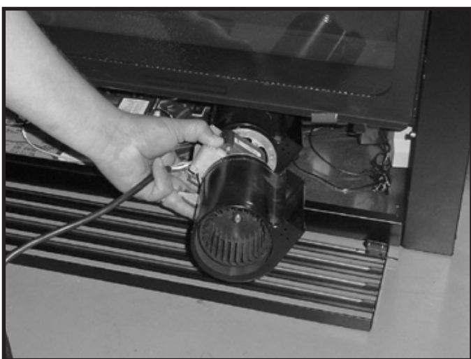
Figure 3 Insert the Fan Into the Appliance (Avoiding Wires)
