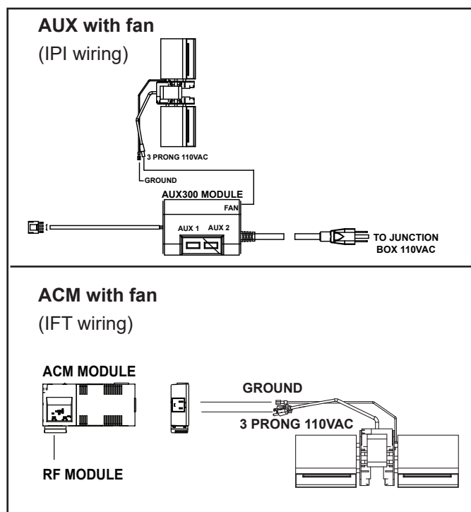
Figure 5 AUX/ACM Wiring
