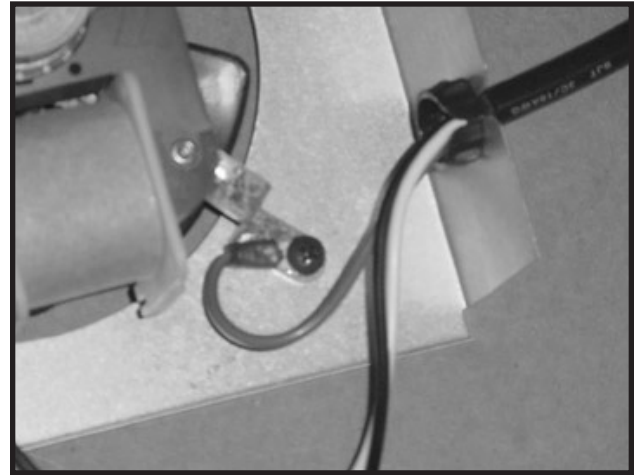
Figure 5 Grounding
